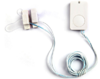
Droplet Duo Sensor Body: 57mm x 35mm x 15.2mm Sensor Probes: 43mm x 13mm x 12mm
